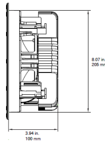
MOUNTING DEPTH/ MINIMUM CUTOUT
